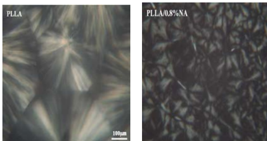
Fig. 4: POM images of PLLA and PLLA/0.8%NA during isothermal crystallization at 115°C.
