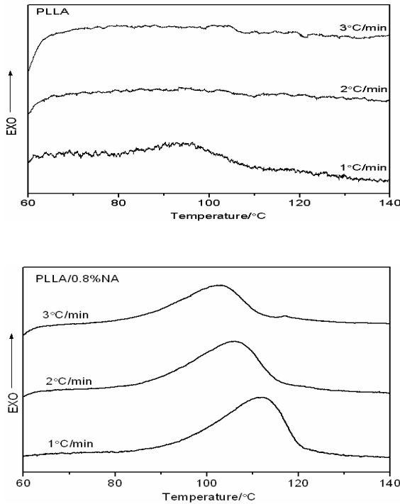
Fig. 3: The non-isothermal crystallization exotherms of PLLA and PLLA/0.8%NA sample from the melt at different cooling rates.
