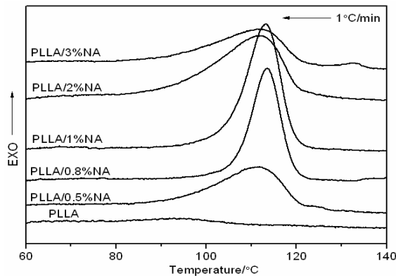
Fig. 1: DSC of PLLA and PLLA/NA crystallized from melt at a cooling rate of 1°C/min
