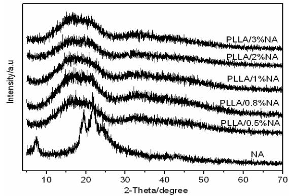
Fig. 2: WAXD patterns of NA and PLLA/NA samples.
